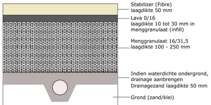
Doorsnede Stabilizer / Stabilizer Fibre
